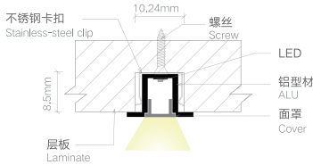
安装节点图 JOINT DRAWING
