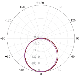
配光曲线 CANDLE POWER DISTRIBUTION CURVE
