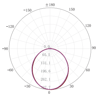
配光曲线 CANDLE POWER DISTRIBUTION CURVE
