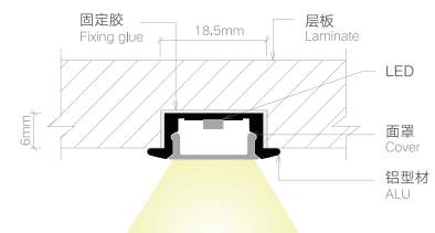
安装节点图 JOINT DRAWING
