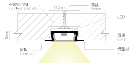
安装节点图 JOINT DRAWING
