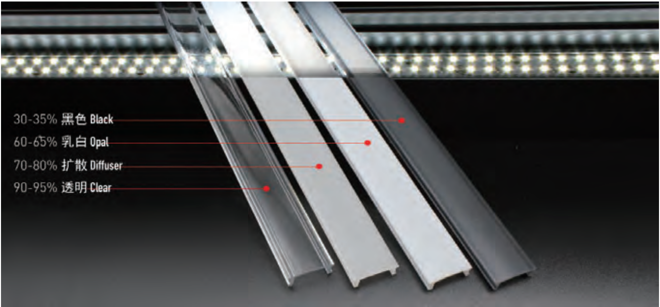
PC面罩常规有四种颜色可选，满足不同应用场景的使用需求 The PC cover is generally available in four colors to meet the needs of different application scenarios.
