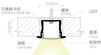
安装节点图 JOINT DRAWING
