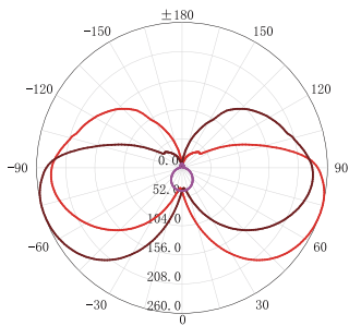
配光曲线 CANDLE POWER DISTRIBUTION CURVE
