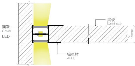
安装节点图 JOINT DRAWING
