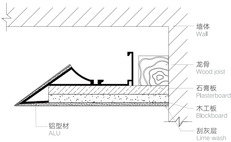
安装节点图 JOINT DRAWING
