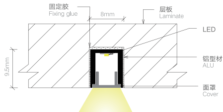
安装节点图 JOINT DRAWING
