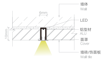
安装节点图 JOINT DRAWING
