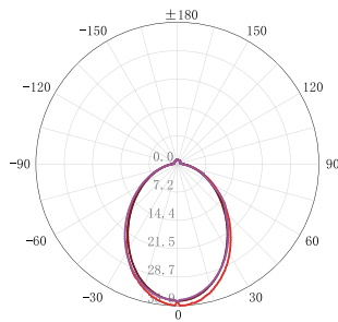
配光曲线 CANDLE POWER DISTRIBUTION CURVE
