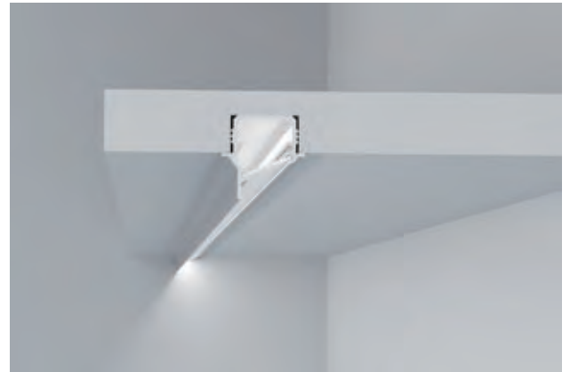
安装节点图 JOINT DRAWING
