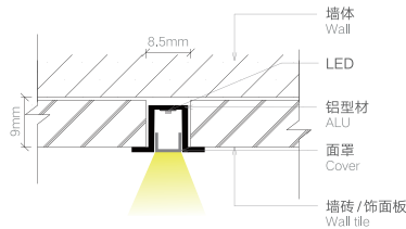
安装节点图 JOINT DRAWING
