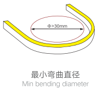
6mm灯带 Strip light 6mm
