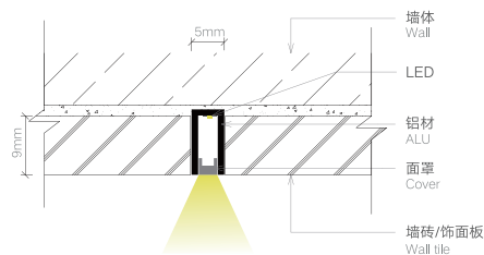
安装节点图 JOINT DRAWING
