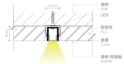
安装节点图 JOINT DRAWING
