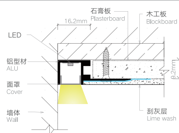
安装节点图 JOINT DRAWING
