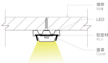
安装节点图 JOINT DRAWING
