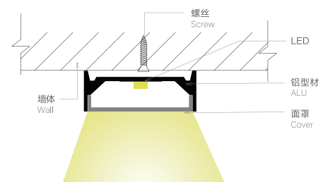
安装节点图 JOINT DRAWING
