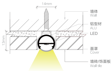
安装节点图 JOINT DRAWING
