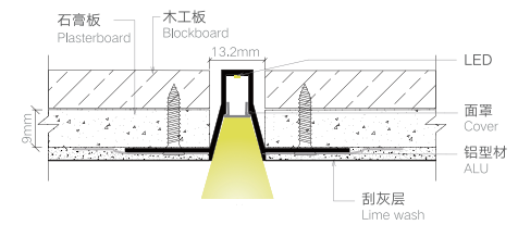
安装节点图 JOINT DRAWING
