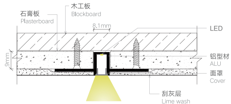
安装节点图 JOINT DRAWING
