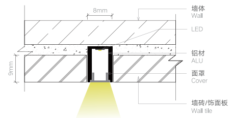
安装节点图 JOINT DRAWING
