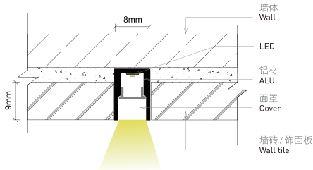
安装节点图 JOINT DRAWING
