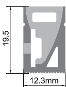
10mm灯带 Strip light 10mm
