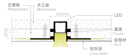
安装节点图 JOINT DRAWING
