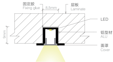
安装节点图 JOINT DRAWING
