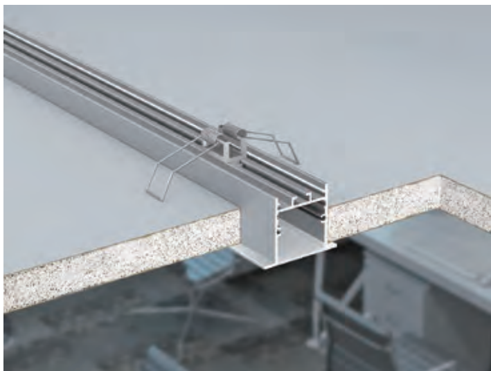
弹簧卡扣 Spring clips
